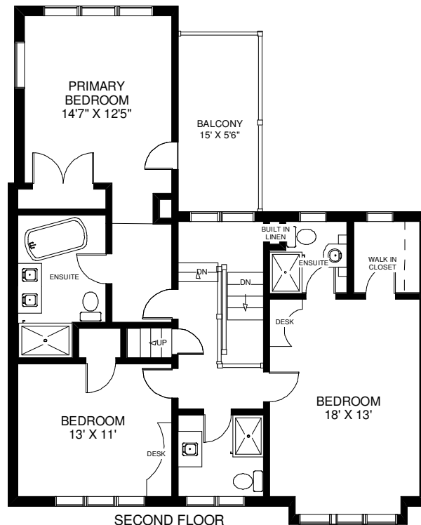
SECOND FLOOR APPROXIMATELY 1,150 SQ FT
