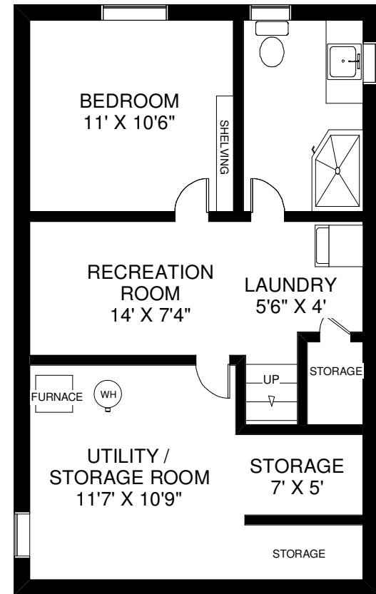
LOWER FLOOR APPROXIMATELY 625 SQ FT
